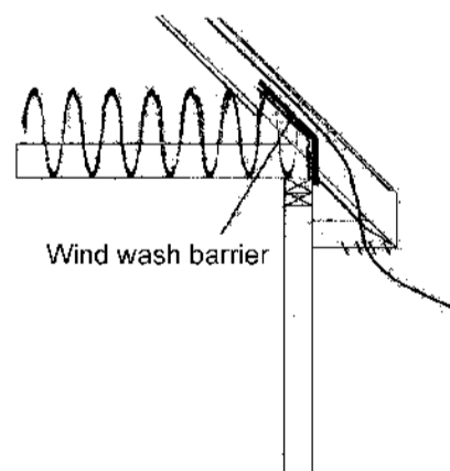
780 CMR FIGURE 6106.3.3.1 WIND WASH BARRIER
