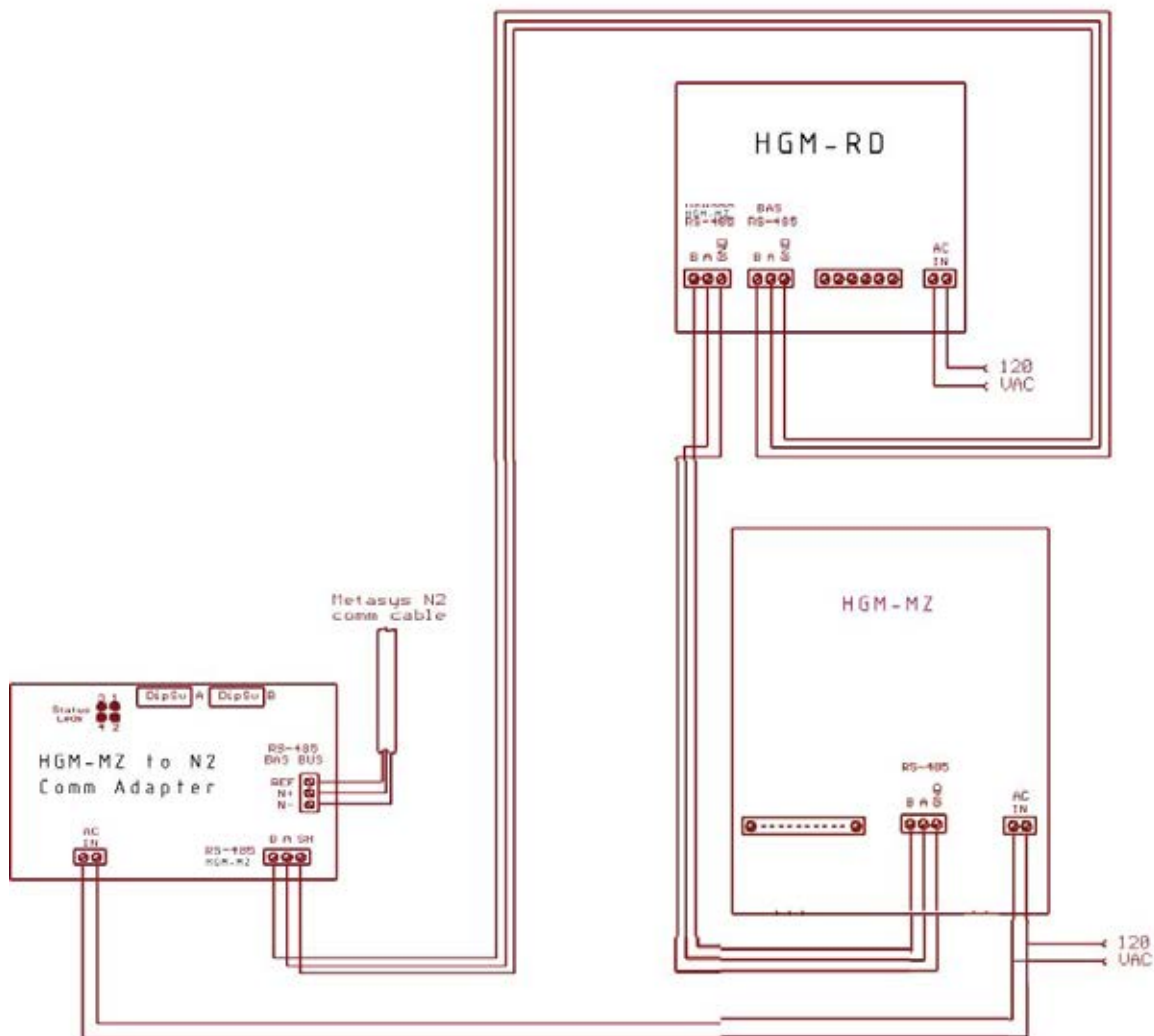
Figure 2 – HGM-MZ to N2 Communications Adapter: Wiring w/Remote Display
