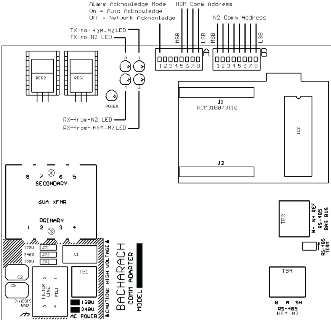
Figure 3 – HGM-MZ to Metasys N2 Adapter: Dipswitches and LED Indicators
