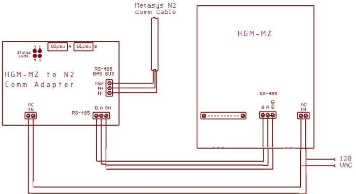
Figure 1 – Wiring w/o Remote Display
