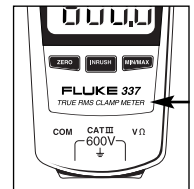
Figure 4. The true-rms clamp is labeled on the front panel.
