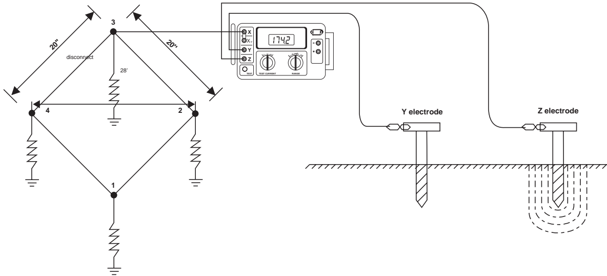
Figure 3. Three-Point test connection
